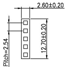
HOUSING
